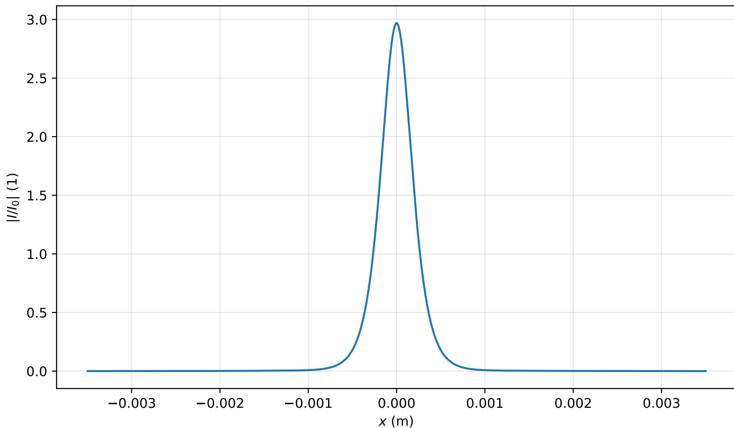
Intensity profile I(x, y = 0, z = 3.503m)/I_0 , P_{in}=1.0P_{cr} , artificial time
